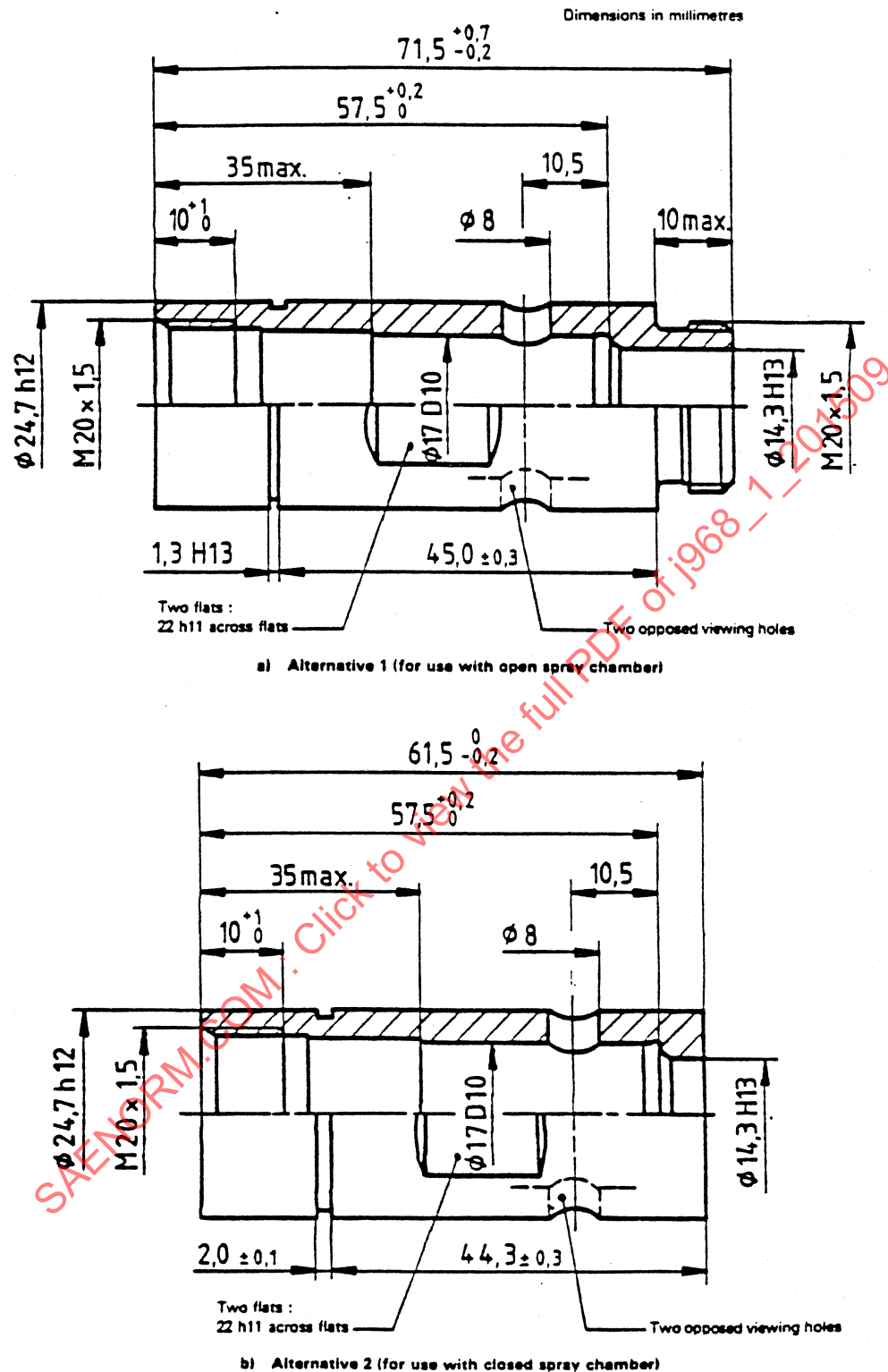
FIGURE 10—RETAINING NUTS (CAPNUTS) FOR CALIBRATING NOZZLE AND HOLDER ASSEMBLY WITH SINGLE HOLE ORIFICE PLATE
