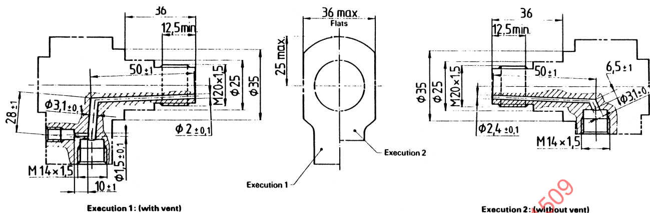
FIGURE 3—HOLDER BODY
