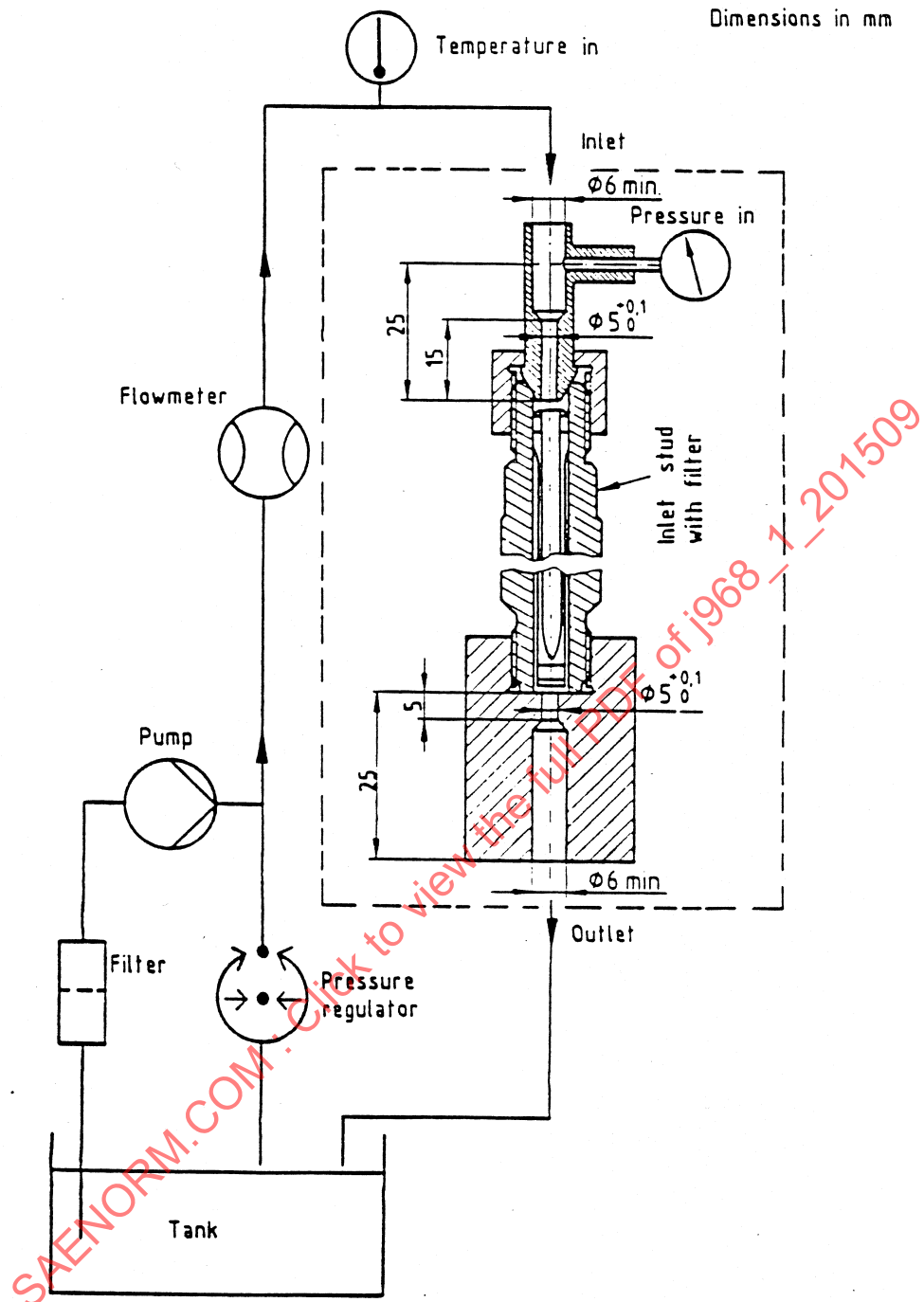
FIGURE 6—INLET STUD FLOW MEASURING SYSTEM
