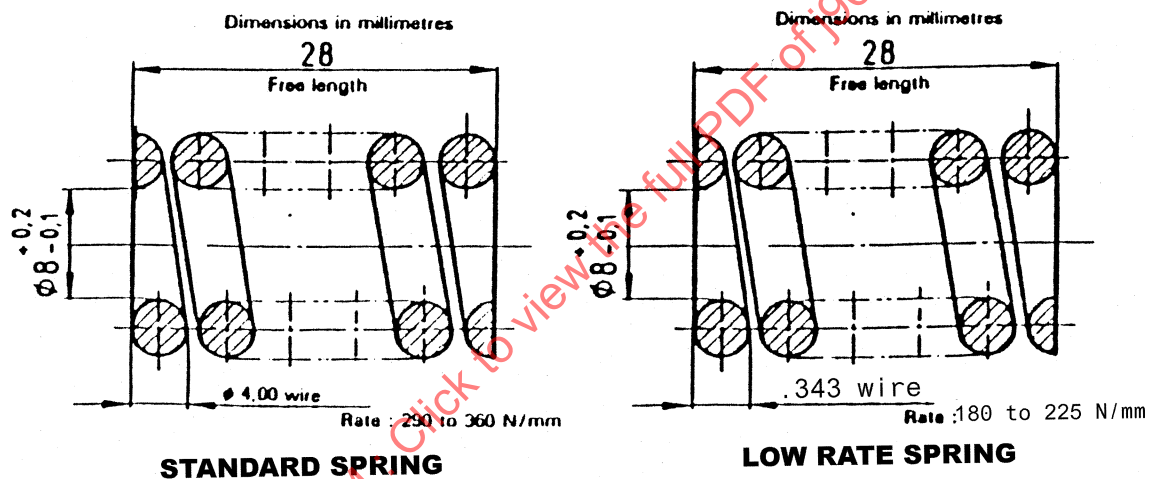
FIGURE 4—SPRINGS
