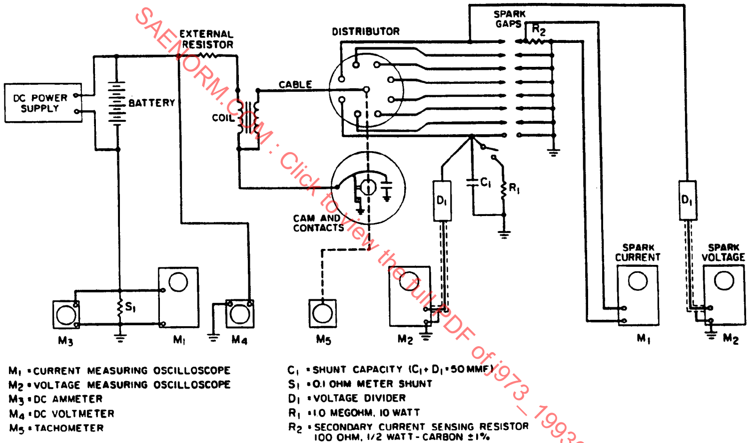
FIGURE 1—TEST CIRCUIT ARRANGEMENT FOR GROUP A TESTS
