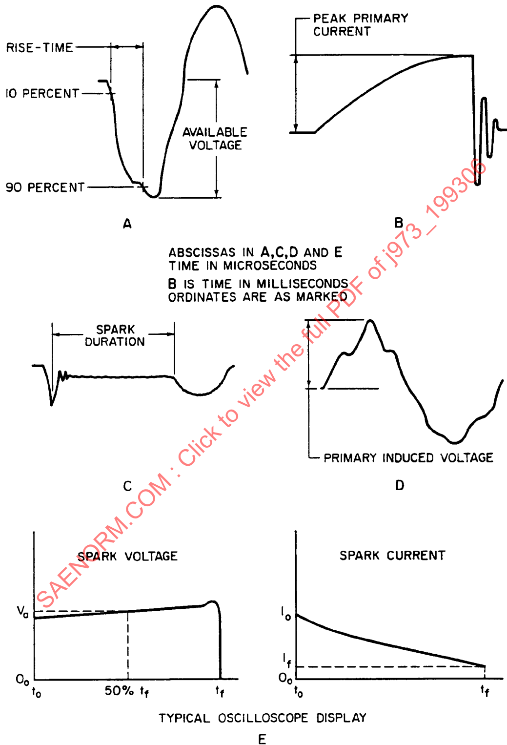
FIGURE 2—TEST CIRCUIT WAVEFORMS
