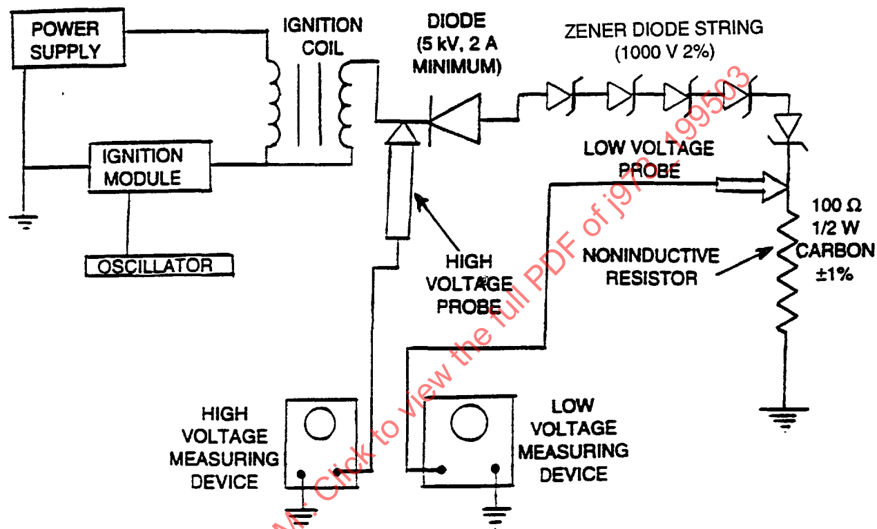
(R) FIGURE 4—IGNITION COIL ENERGY MEASUREMENT (ZENER TECHNIQUE)
