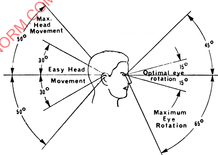
FIGURE 4—VERTICAL EXTENT OF HEAD AND EYE MOVEMENT
