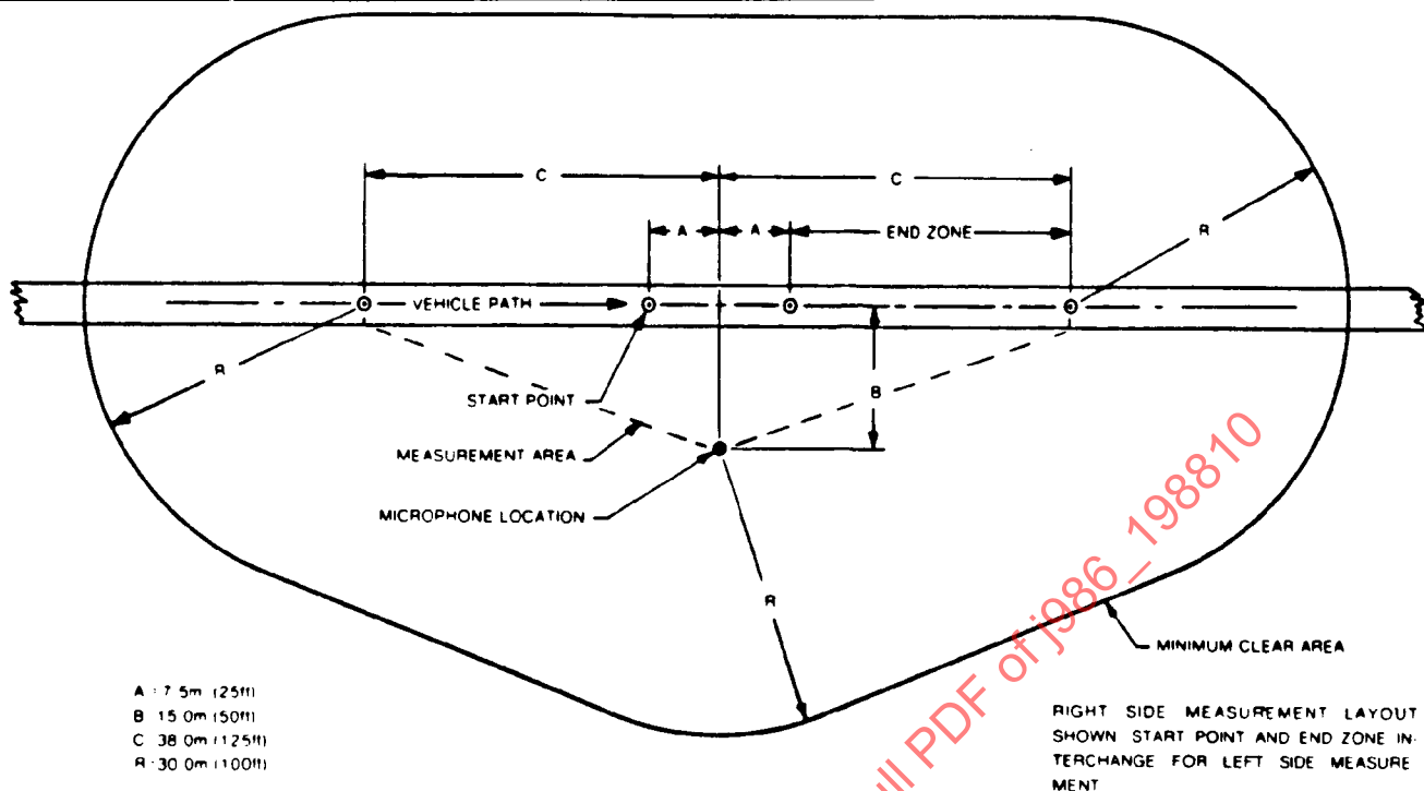
FIGURE 1 - Minimum Test Site
