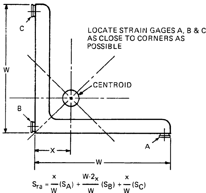
FIG. 4—WEIGHTING TEST DATA FOR AVERAGE AXIAL STRESS
