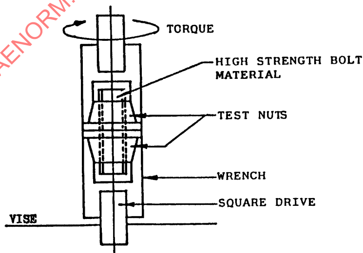
FIGURE B1 - Wrench Torque Test Apparatus
