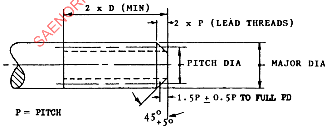
FIGURE E2 - Minimum Mandrel
