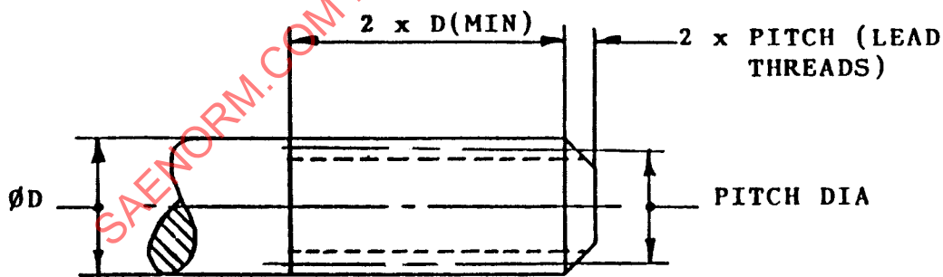
FIGURE E1 - Maximum Mandrel
