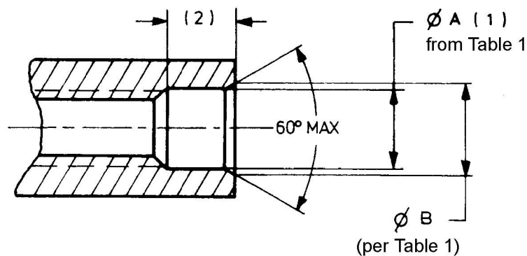
FIGURE 2 - Tapped Hole Centers
