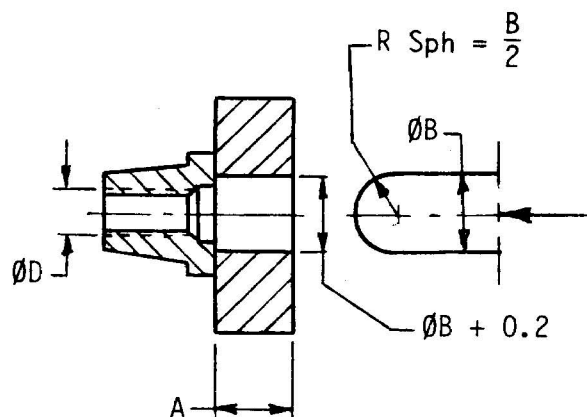
FIGURE C2 - Push Out Test Apparatus
