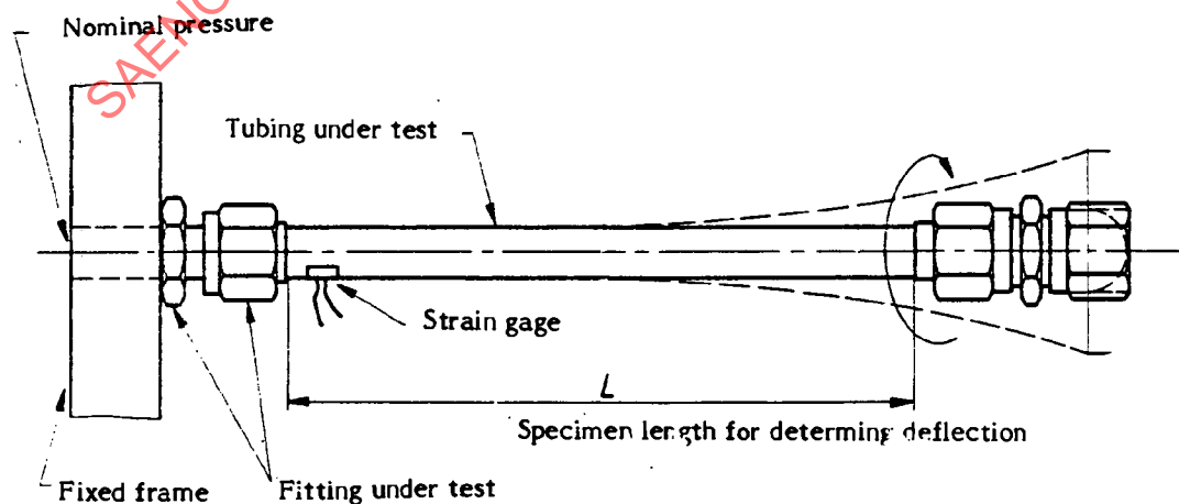
Figure 1 - Schematic for Flexure Test Specimen
