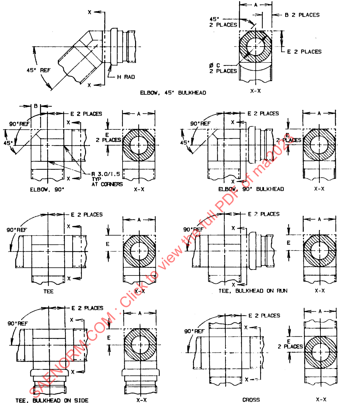
FIGURE 1 STANDARD AND REDUCED ENVELOPE FITTINGS
