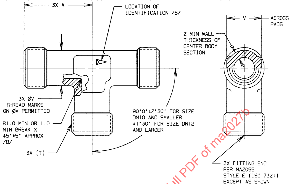
FIGURE 1 TEE, FLARELESS
