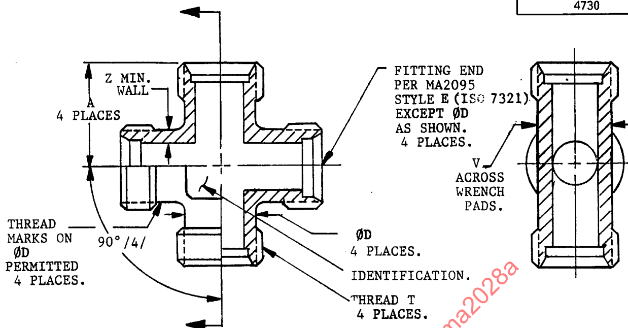
FIGURE 1 - FRONT AND SIDE VIEWS
