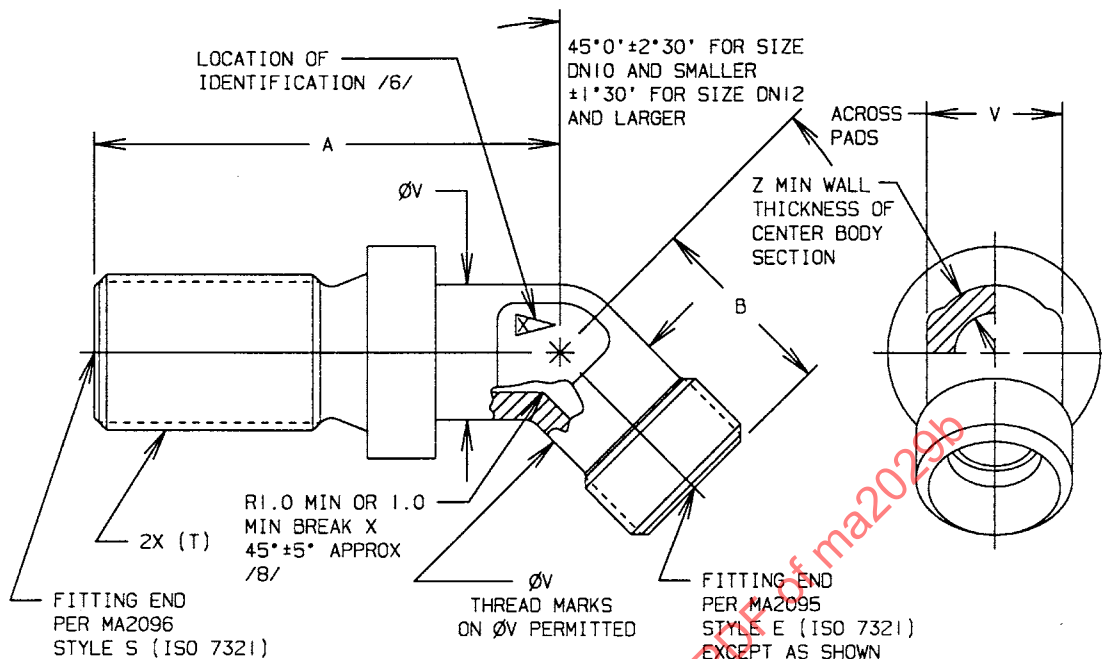
FIGURE 1 ELBOW, 45°, FLARELESS
