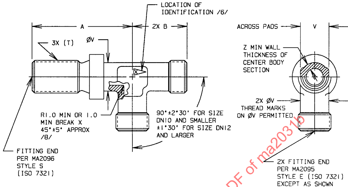
FIGURE 1 TEE, FLARELESS
