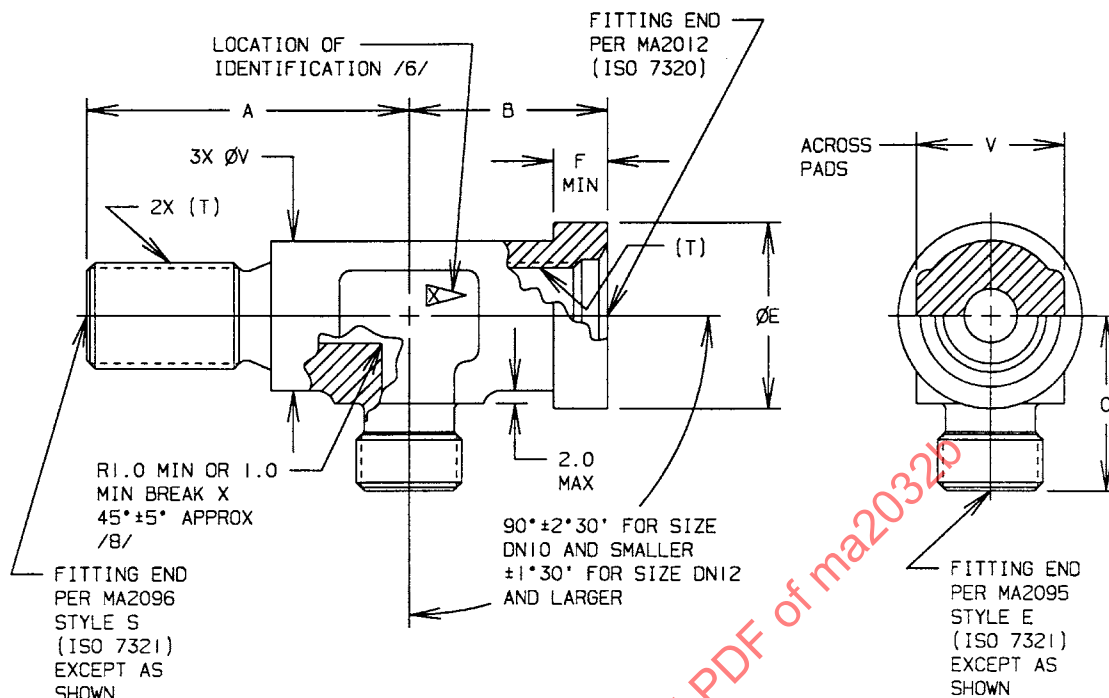
FIGURE 1 TEE, FLARELESS
