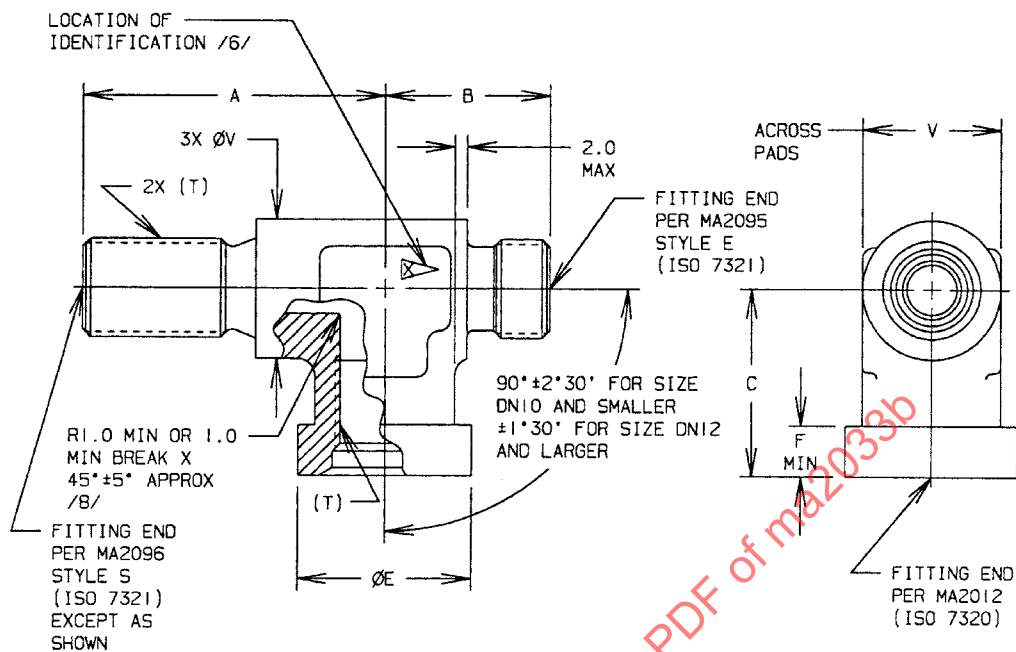
FIGURE 1 TEE, FLARELESS
