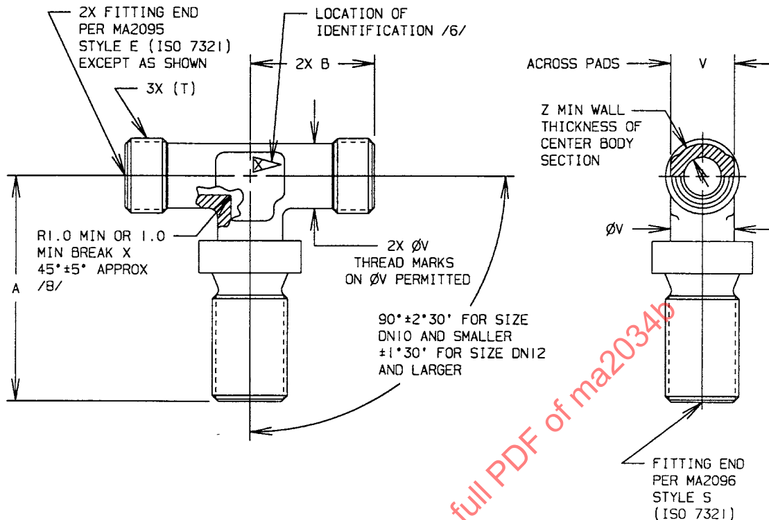
FIGURE 1 TEE, FLARELESS
