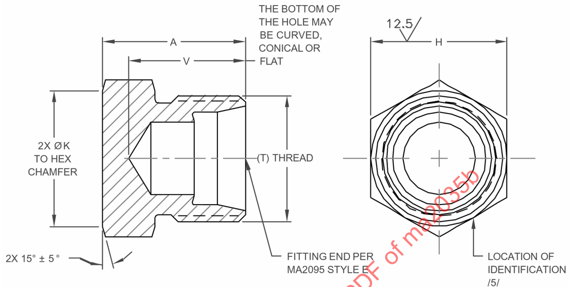
FIGURE 1 - PLUG
