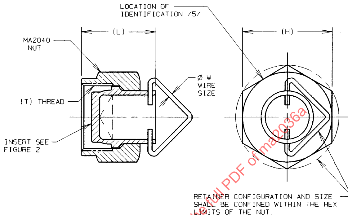
FIGURE 1 - CAP ASSEMBLY
