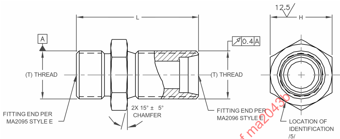
FIGURE 1 - UNION, BULKHEAD
