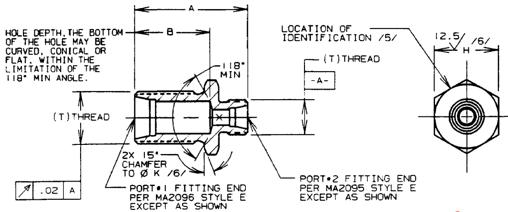
FIGURE 1 - UNION, REDUCER, BULKHEAD, FLARELESS END SHOWN AS REDUCER
