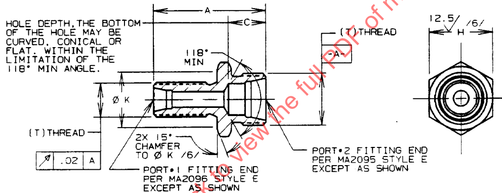
FIGURE 2 - UNION, EXPANDER, BULKHEAD, BULKHEAD END SHOWN AS REDUCER
