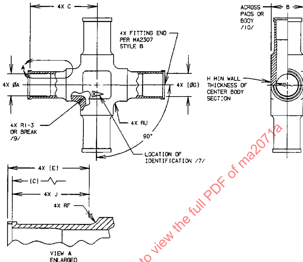
FIGURE 1 - FITTING, CROSS
