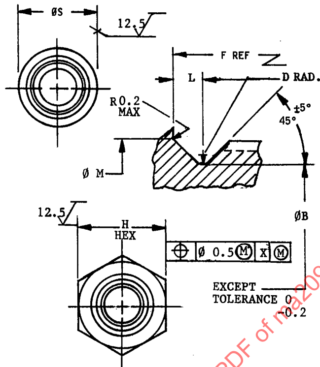
FIGURE 3 - ENLARGED VIEW B
