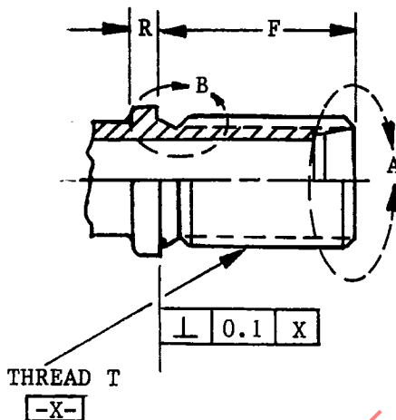
FIGURE 1 - FRONT AND SIDE VIEWS FOR STYLE S
