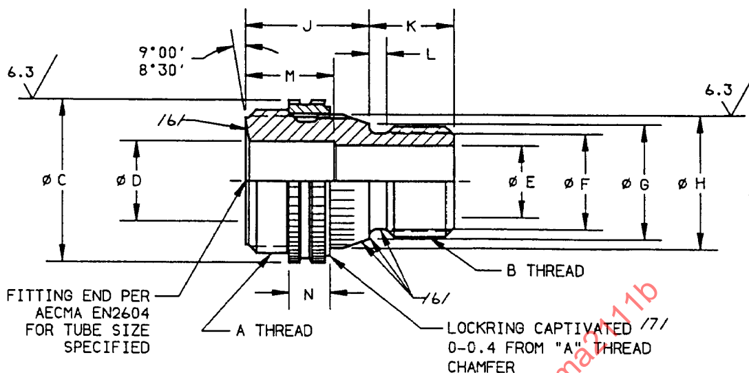
FIGURE 1 - ADAPTER, ASSEMBLY
