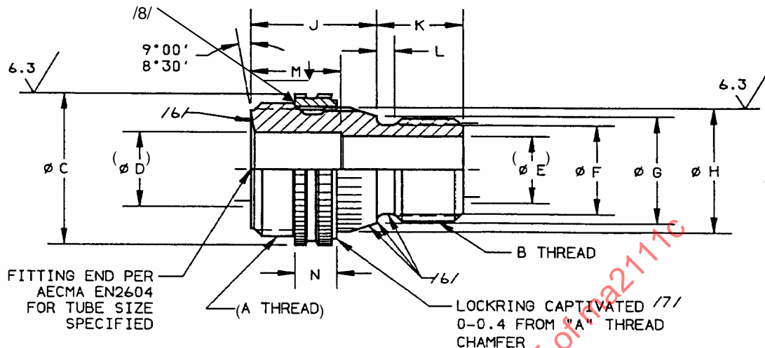
FIGURE 1 - ADAPTER, ASSEMBLY
