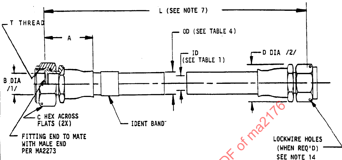
FIGURE 1 - DETAIL OF HOSE ASSEMBLY
