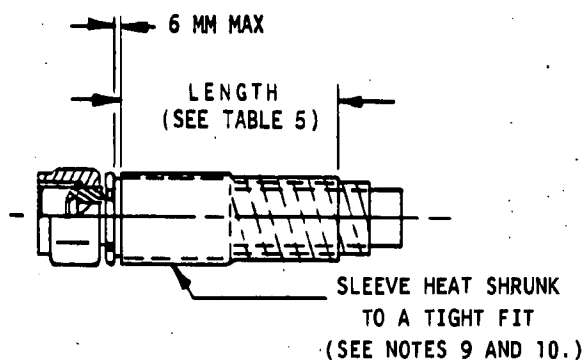
FIGURE 2 - DETAIL OF SLEEVE ASSEMBLY
