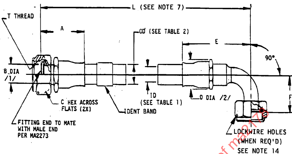
FIGURE 1 - Detail of Hose Assembly
