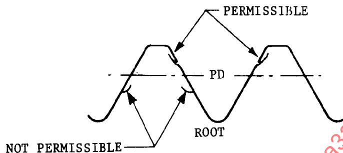
LAPS EXTENDING TOWARDS CREST, ROLLED THREAD FIGURE 7
