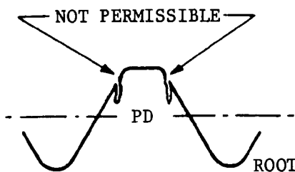
MULTIPLE LAPS ABOVE PD EXTENDING TOWARD ROOT, ROLLED THREAD FIGURE 4
