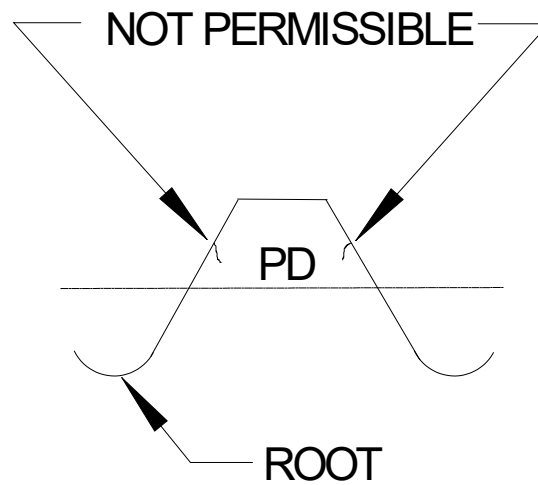
Figure 4 - Laps above PD extending toward root, rolled thread
