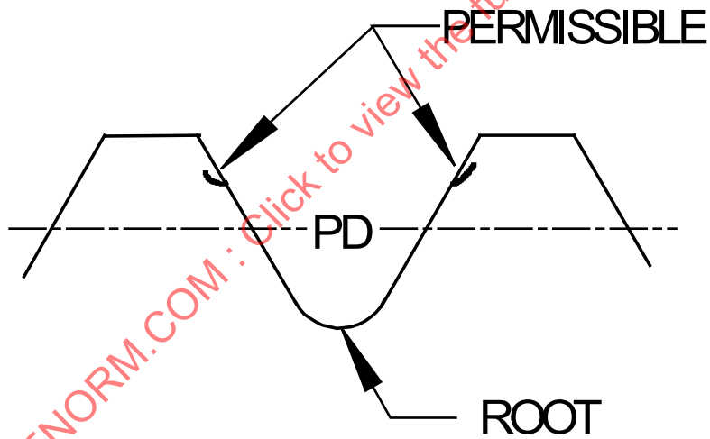
Figure 3 - Laps above pitch diameter extending towards crest, rolled thread
