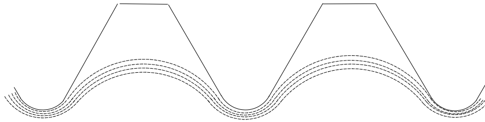
Figure 1 - Flow lines, rolled thread
