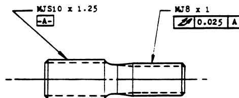
VIEW G
