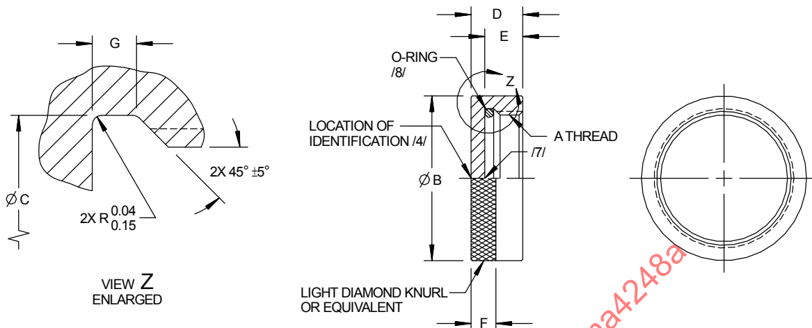
FIGURE 1 - CAP ASSEMBLY
