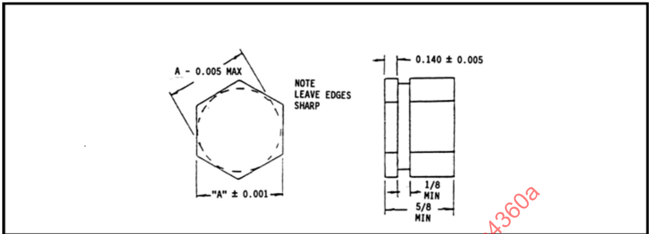
FIGURE 2 - SPECIMEN FOR ALUMINUM MANDREL TEST
