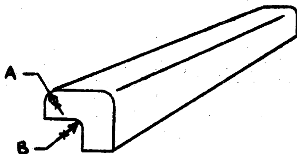
CORNER AND FILLET RADII DIMENSIONS
