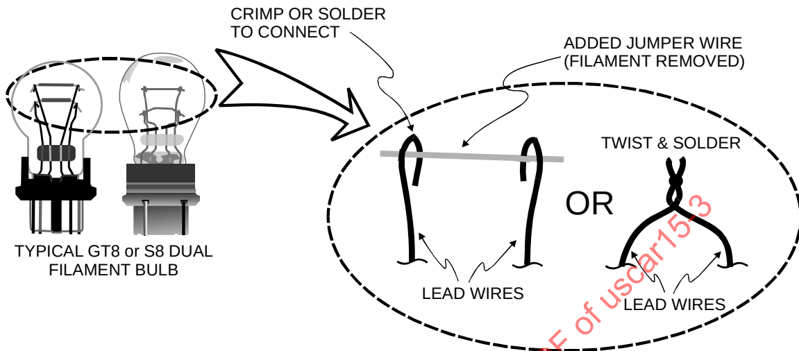
S8/GT8 Voltage Test Device Figure
