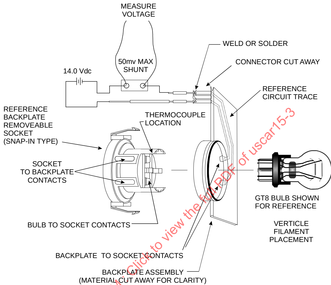
Figure 3-A: Vibration: Continuity and Temperature Monitoring (Socket design shown for reference only)
