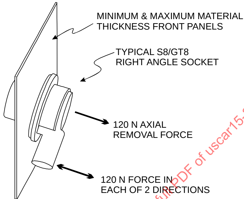
Figure 7: Socket Strength (Right Angle)
