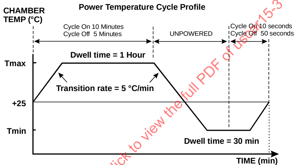
Figure 11: Power Temperature Cycle Profile Criteria
