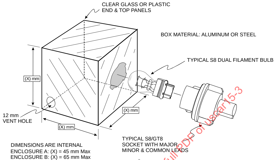
Figure 6: Outgassing Separate socket shown. Enclosure for circuit plate assembly to accommodate that design.
