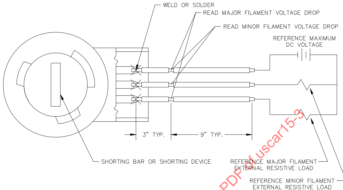
Voltage Drop Circuit Diagram Figure
