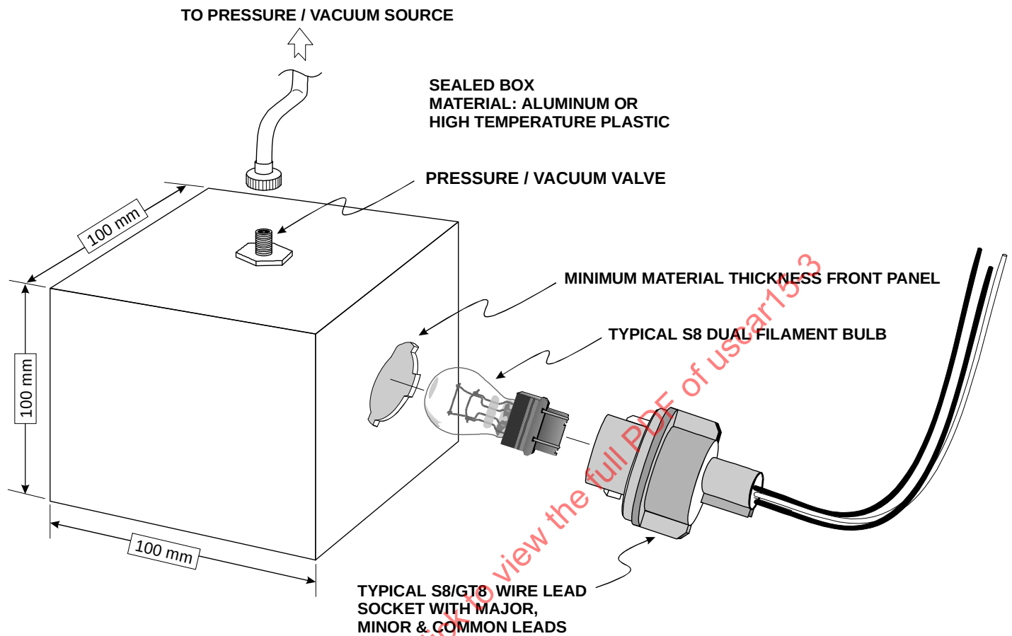
Figure 4: Socket Pressure/Vacuum Test Fixture
