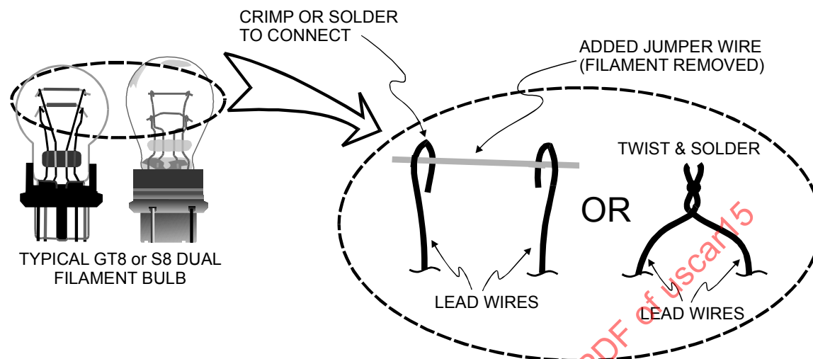
S8/GT8 Voltage Test Device Figure
