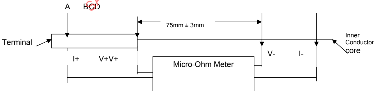
Figure 4.4.4.4-a: Center conductor dry circuit measurement points
