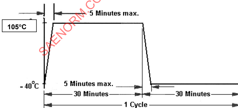
6 Figure 2.4: Thermal Shock Programming and Operation
