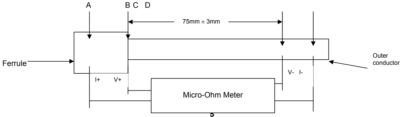
Figure 4.4.4.4-b: Outer conductor dry circuit measurement points
