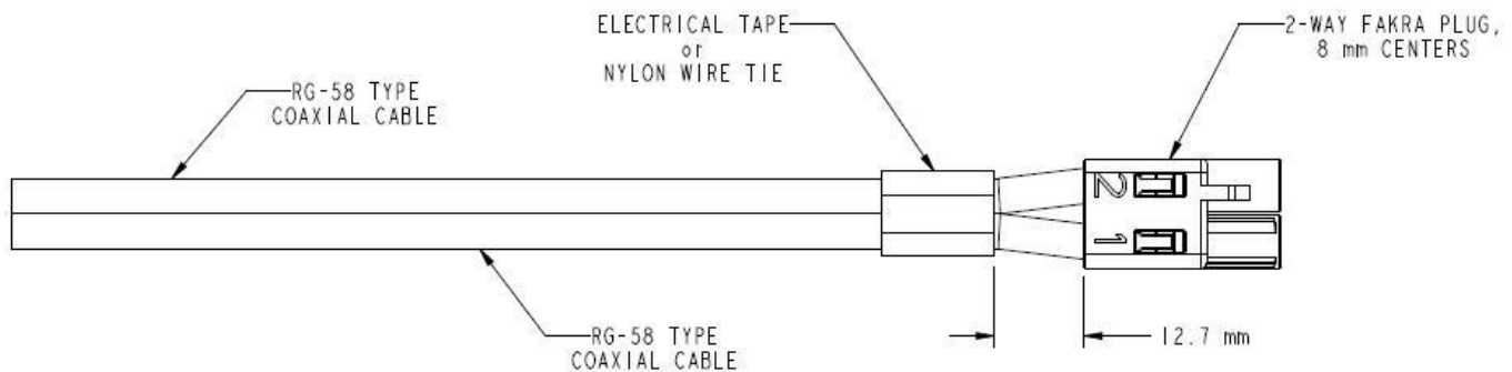
FIGURE 4.2.2.2.3.B Male Connector Constrained
