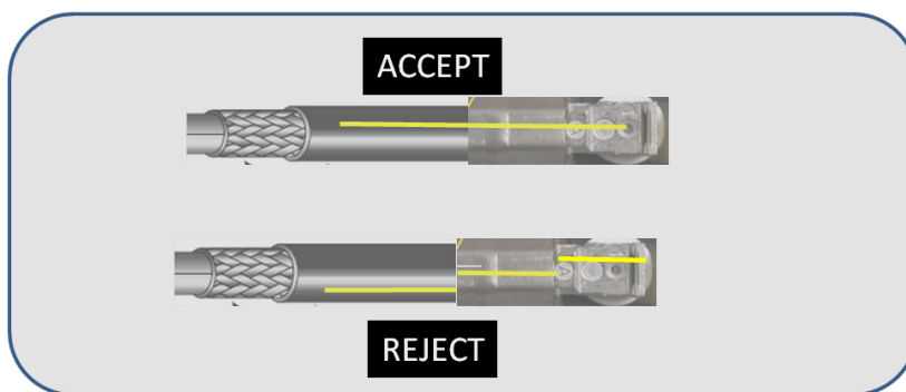
Figure 4.2.6.5-A: Torque Criteria
