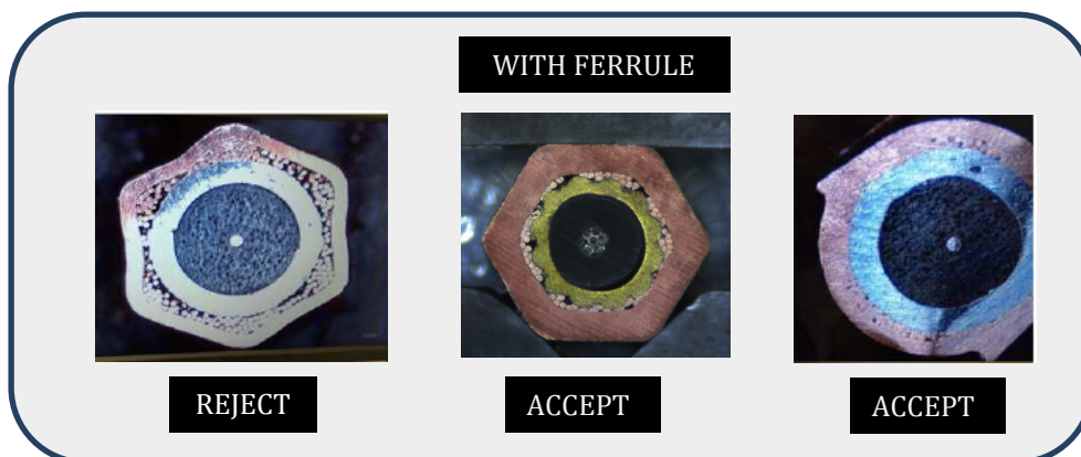
Figure 4.2.6.5-C: Crimp Criteria
