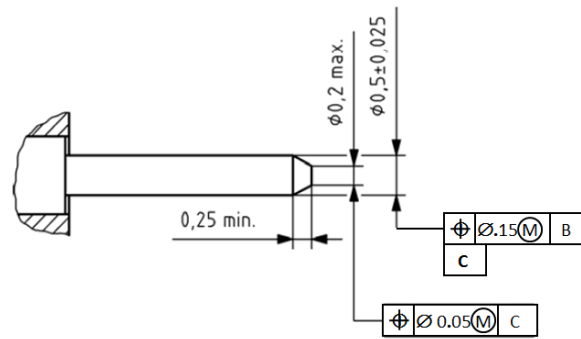
Figure 2X - Pin Dimensions
