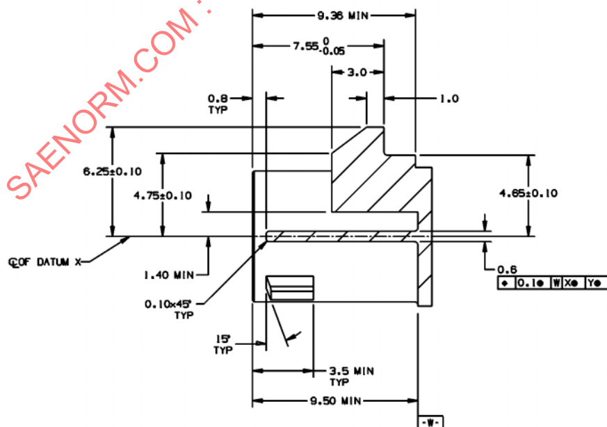
FIGURE 4.2.2: Latch Detail
