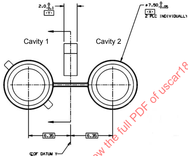
FIGURE 4.2.1: Cavity Detail (Coding C2 Shown)
