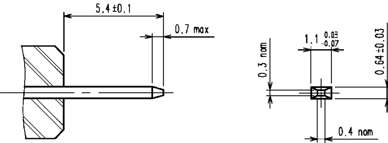
FIGURE 3.2: Male Terminal Dimensioning Requirements
