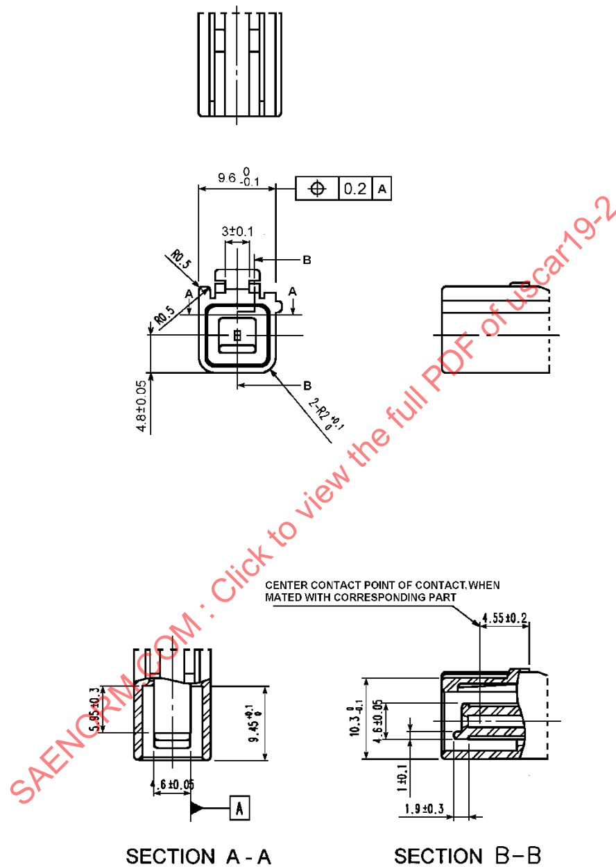
FIGURE 4.1: Reference Dimensions of the Plug
