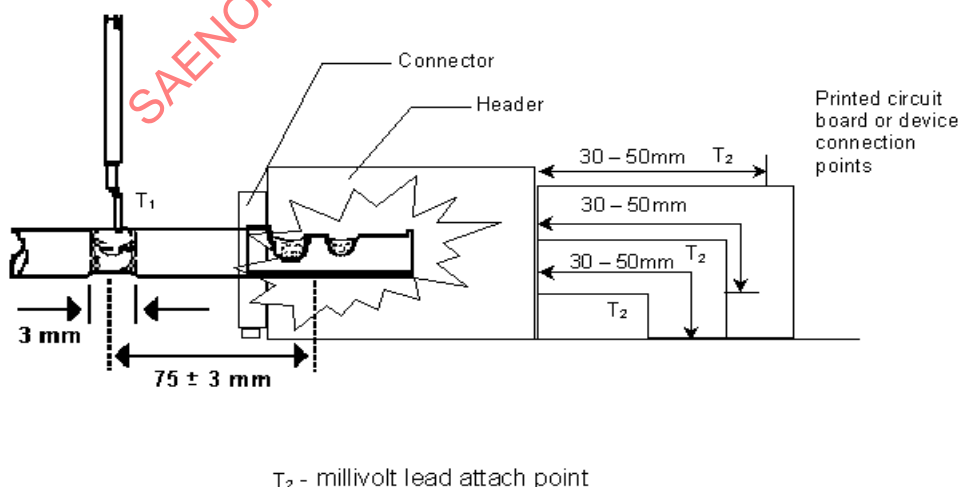
FIGURE 5.1.5: MILLIVOLT LEAD ATTACHMENT (TYPICAL)
