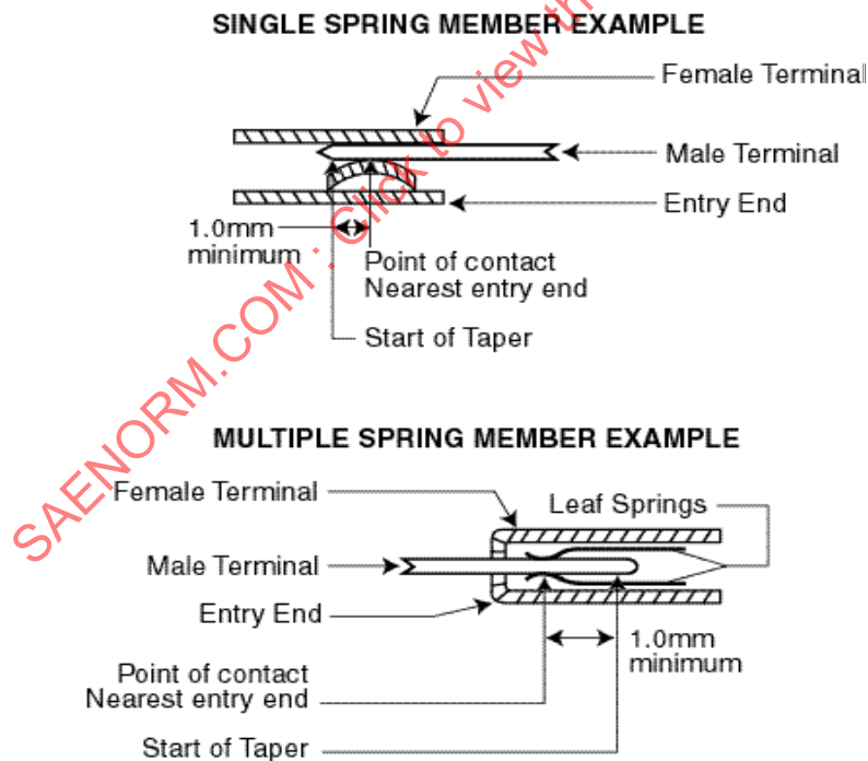
FIGURE 5.3.1.4: TERMINAL INSERTION
