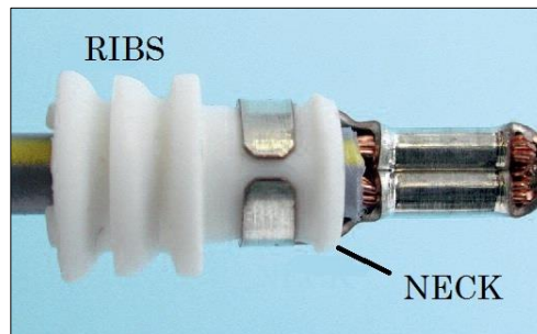
FIGURE 4.2.5H - INDIVIDUAL CABLE SEAL DETAIL
