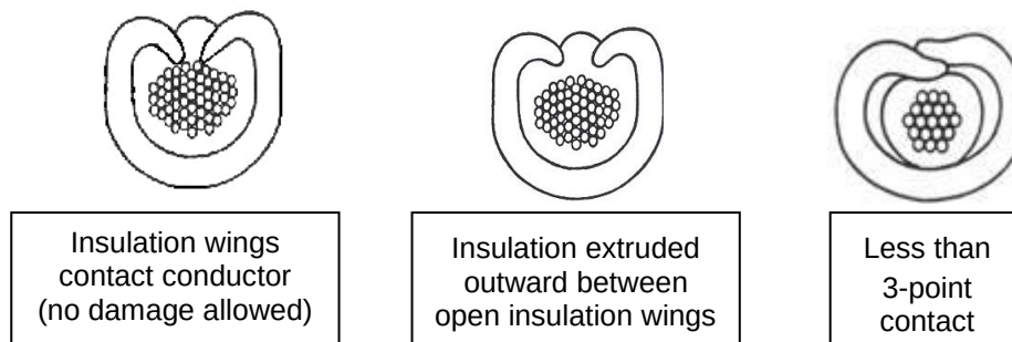
FIGURE 4.3.5-3B - ACCEPTABLE BUT NOT IDEAL INSULATION CRIMPS
