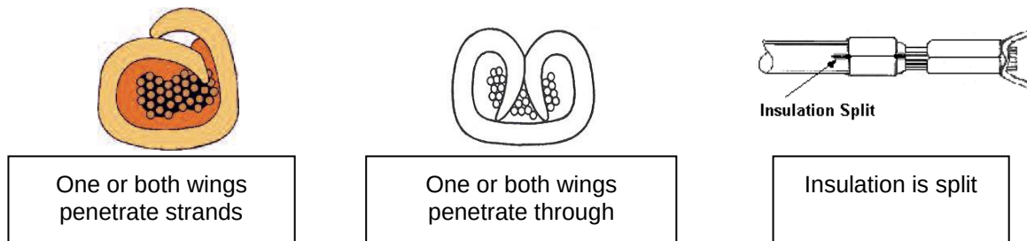
FIGURE 4.3.5-3C - UNACCEPTABLE INSULATION CRIMPS
