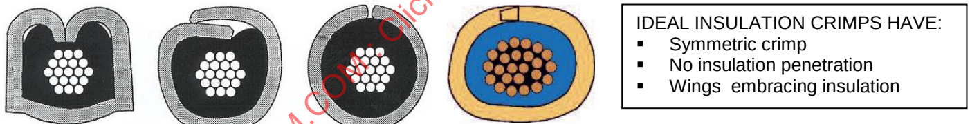
FIGURE 4.3.5-3A - IDEAL INSULATION CRIMP CROSS-SECTIONS FOR DIFFERENT STYLE DESIGNS
