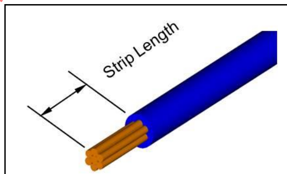
FIGURE 4.2.5G - STRIPPED WIRE LENGTH
