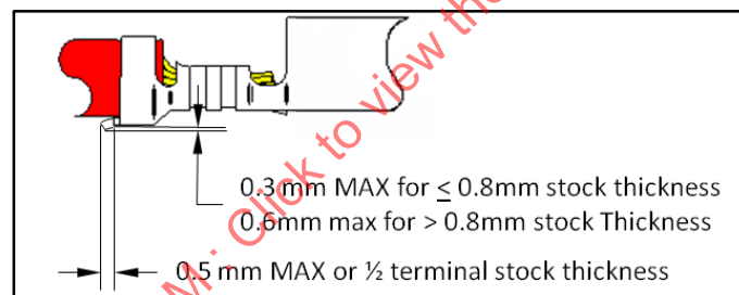
FIGURE 4.2.5C - BURR CRITERIA FOR CUT-OFF TAB
