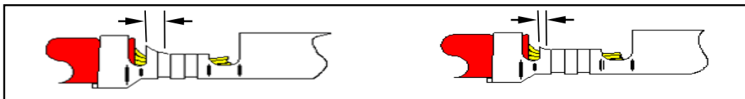
FIGURE 4.2.5D AND 4.2.5E - BELL MOUTH ACCEPTANCE CRITERIA (MAX. AND MIN.)
