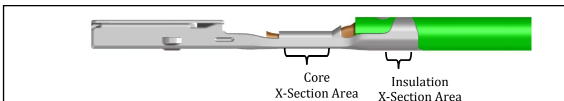
FIGURE 4.3.4-3 - CRIMP CROSS-SECTION LOCATIONS
