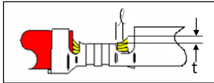
FIGURE 4.2.5F - WIRE BRUSH PROTRUDING STRAND HEIGHT ABOVE CORE CRIMP (t) AND LENGTH (l)
