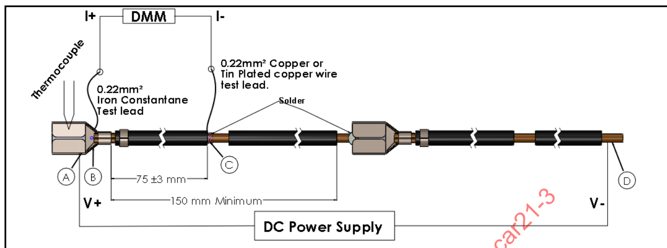
FIGURE 4.5.1.4 - TEST LEAD ATTACHMENT
