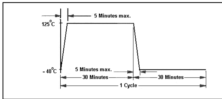
FIGURE 4.5.5.4 - THERMAL SHOCK CYCLE
