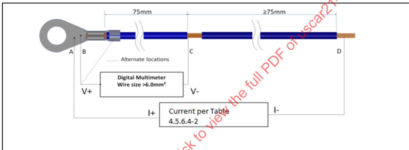
FIGURE 4.5.6.2 - POWER HOOK-UP AND MEASUREMENT POINTS FOR VOLTAGE DROP MEASUREMENT
