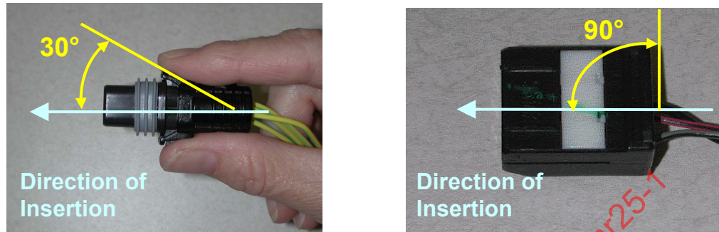
Acceptable Contact Surface: Optimally angled between 30^\circ and 90^\circ from the direction of force insertion
