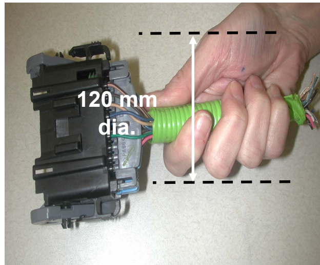
FIGURE 9. HAND GRASP CLEARANCE WITH BUNDLE
