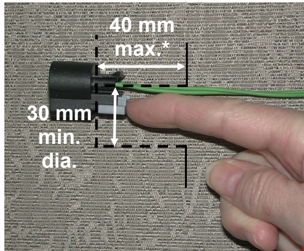
FIGURE 11. ONE FINGER/THUMB PUSH CLEARANCE (SIDE VIEW)
