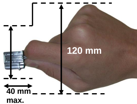
Figure 10B: Hand Grasp Clearance (Top view – Hand in line with Connector)
