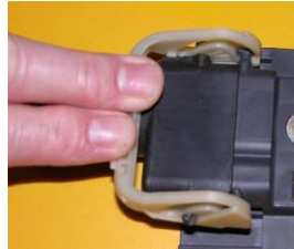
Figure 7: Constrained Lever Lock Connector example: Fingers / thumbs are constrained within the structure of the lever.
