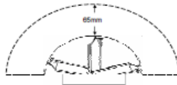
Figure 17: Lever Lock Swing Path and Clearance - Pull
