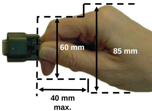
Figure 10A: Hand Grasp Clearance (Side view – Hand in line with connector)
