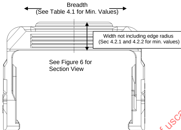
Figure 5: Lever Contact Surface Area
