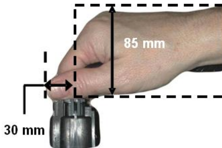
Figure 10C: Hand Grasp Clearance (Side view – Hand 90° to Connector)
