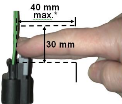
Figure 12A: Two Finger Push Clearance (Side View)
