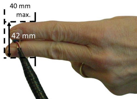
Figure 12B: Two Finger Push Clearance (Top View)
