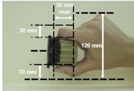
Figure 18: Twist Lock Connector Clearance
