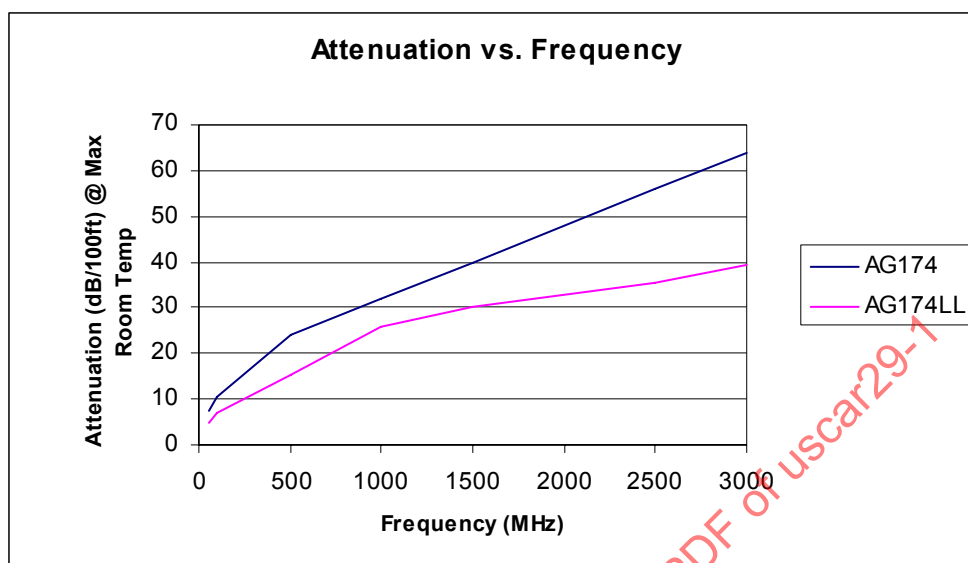
FIGURE 3: Maximum Attenuation Values
