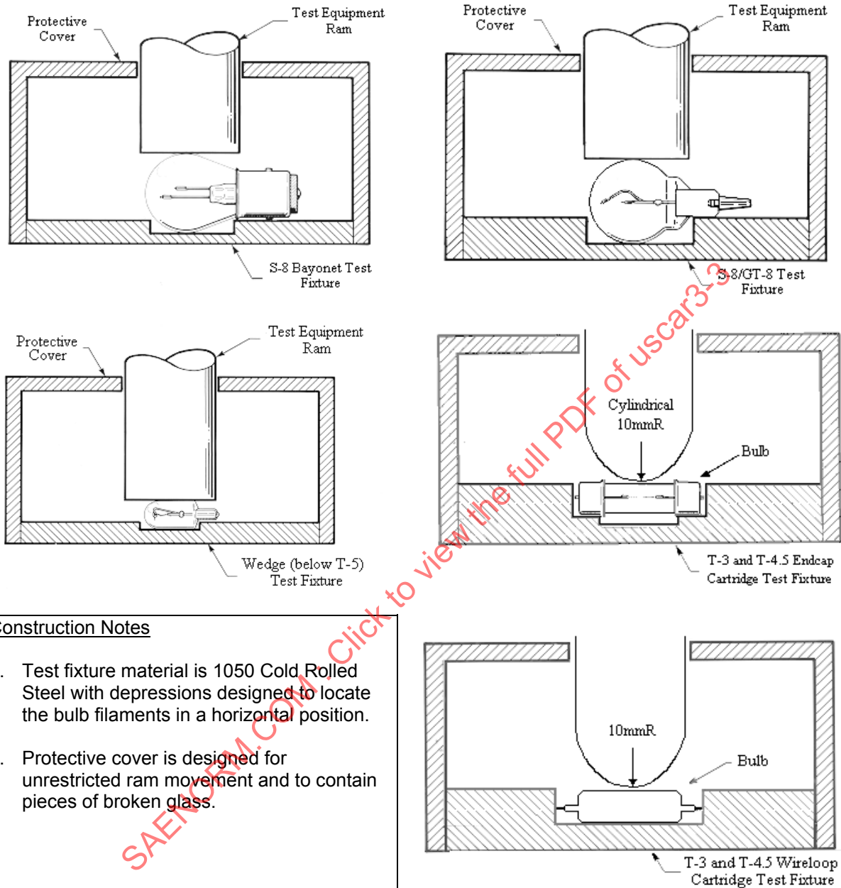
Figure B2 - Crush Test Fixtures
