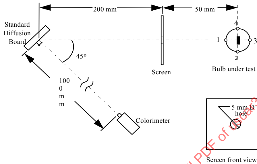
Figure __ b -- SIDE VIEW
