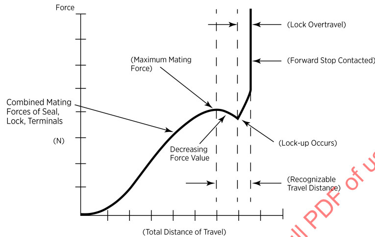
Figure 5.2.1.3: Typical Connector Mating Force Curve
